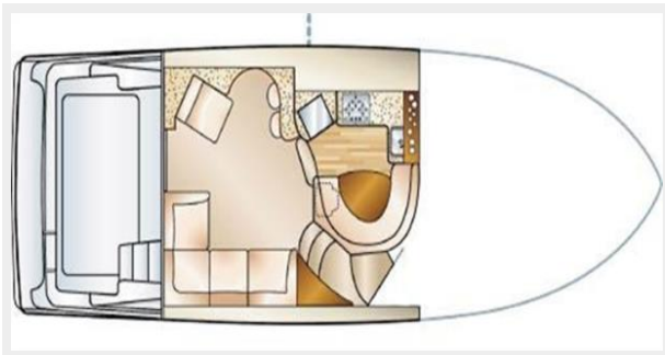
Salon/Galley floorplan
