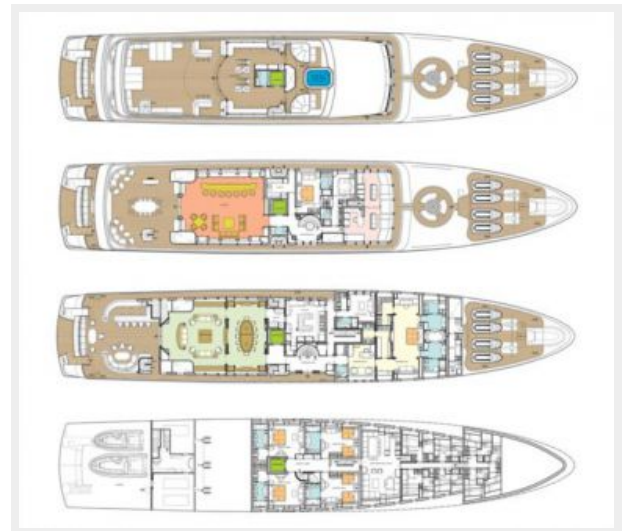
3 Apogee 63m codecasa charter superyacht
