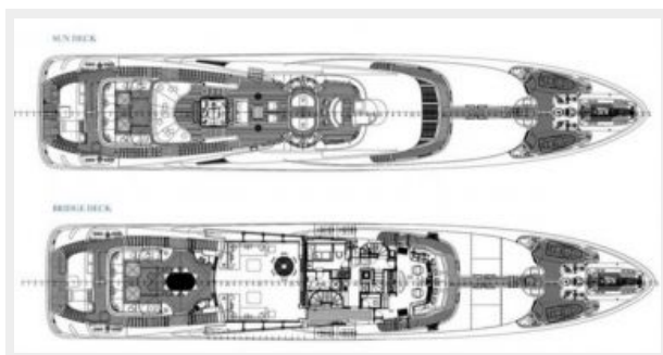
General Arrangement
