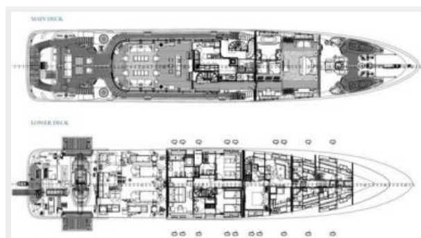
General Arrangement
